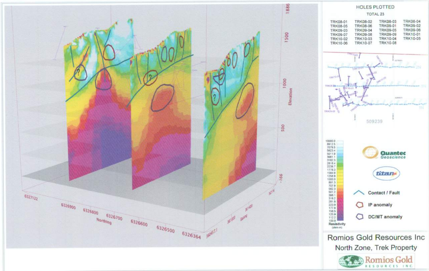
Figure 2-11: Geosoft 3D view of the MT models, with interpretation and DDH.
